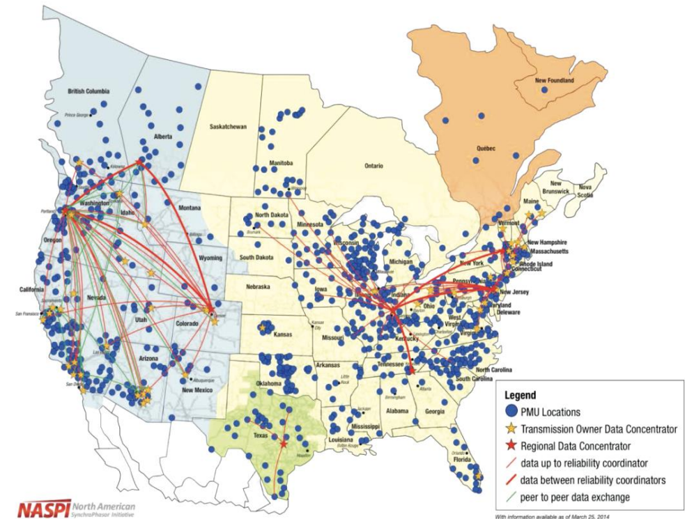
Figure 3.13 Data Flows from Transmission Owners to Regional Hubs, Between Reliability Coordinators, and Between Transmission Operators
